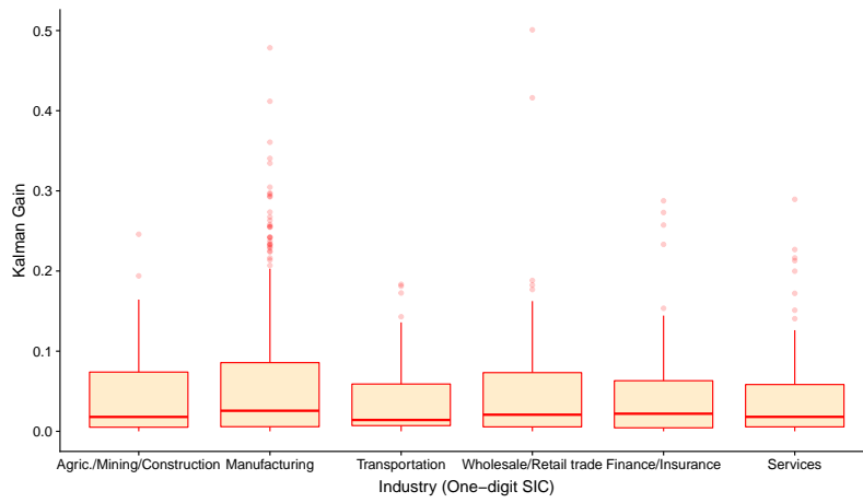
Figure 7: Distribution of Kalman gains by industry
